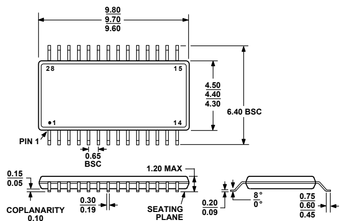
COMPLIANT TO JEDEC STANDARDS MO-153-AE Figure 45. 28-Lead Thin Shrink Small Outline Package [TSSOP] (RU-28) Dimensions shown in millimeters
